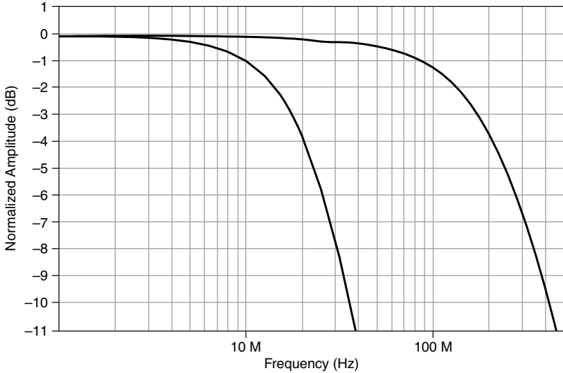
Figure 5. PXIe-5160 Bandwidth-Limiting Filters Frequency Response, 1 V pk-pk , Measured
