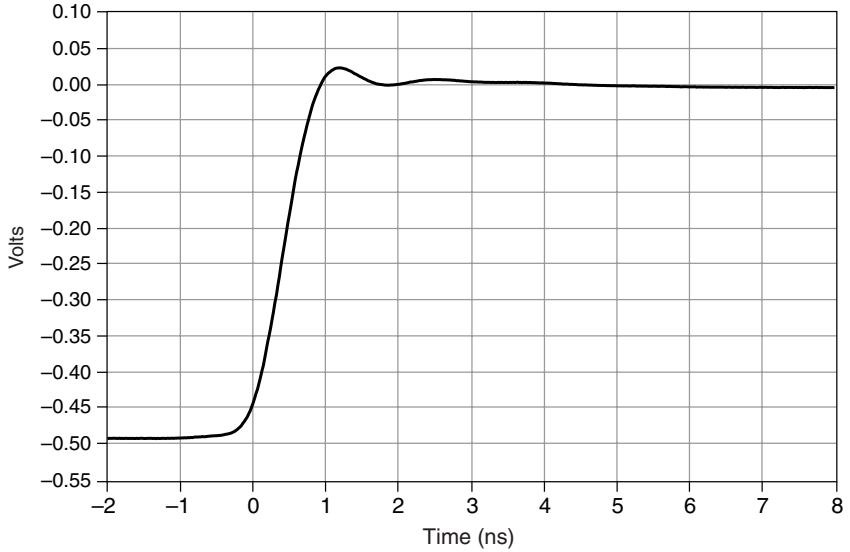
Figure 2. PXIe-5160 Step Response, 1 M \Omega , 1 V pk-pk Input Range, -0.25 V Programmable Offset, 500 ps Rising Edge, Measured 17
