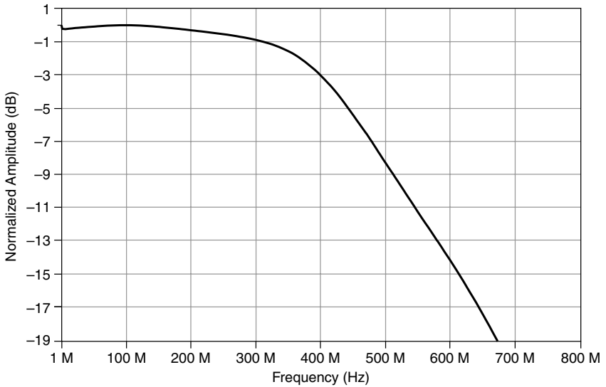
Figure 4. PXIe-5160 1 M \Omega Frequency Response, 1 V pk-pk , Measured 18
