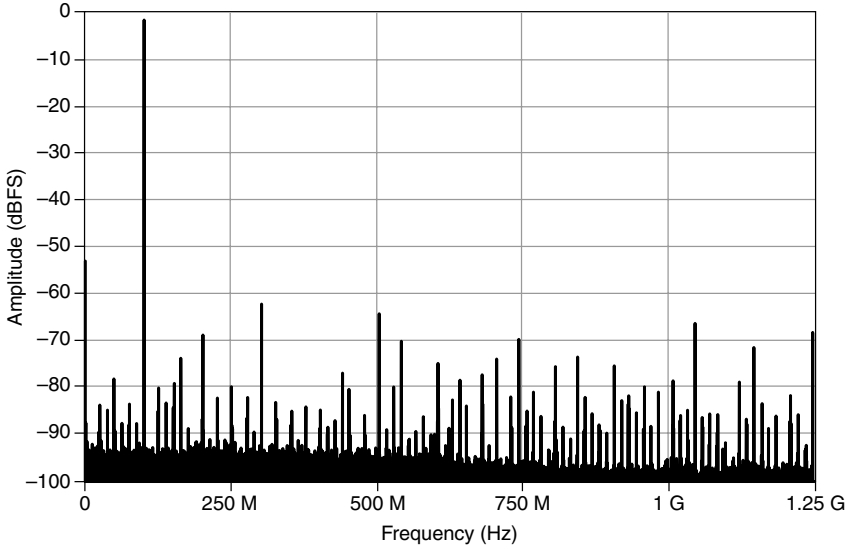
Figure 6. PXIe-5160 Single Tone Spectrum, 2.98 dBm Input Signal at Connector, 50 \Omega , 1 V pk-pk , 2.5 GS/s, 101 MHz Input Tone, Full Bandwidth, Measured
